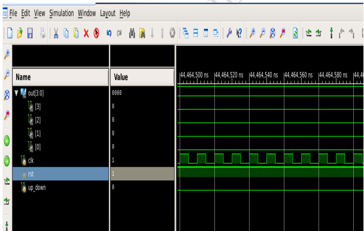
Output waveform:-4 bit up down counter when rst=1 and up_down=0
