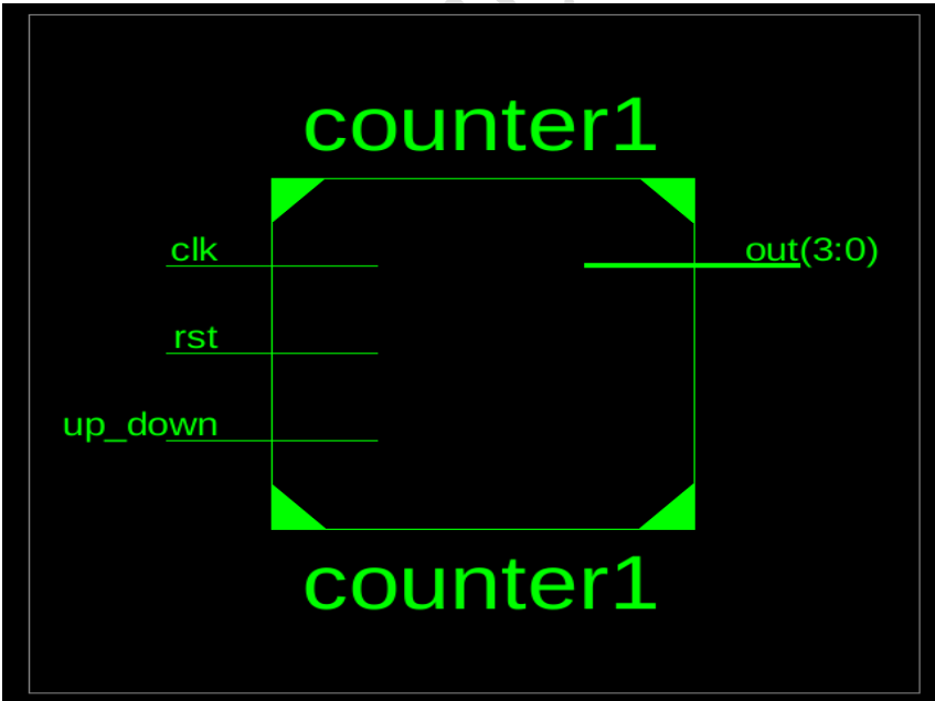
RTL schematic:- 4 bit Counter
