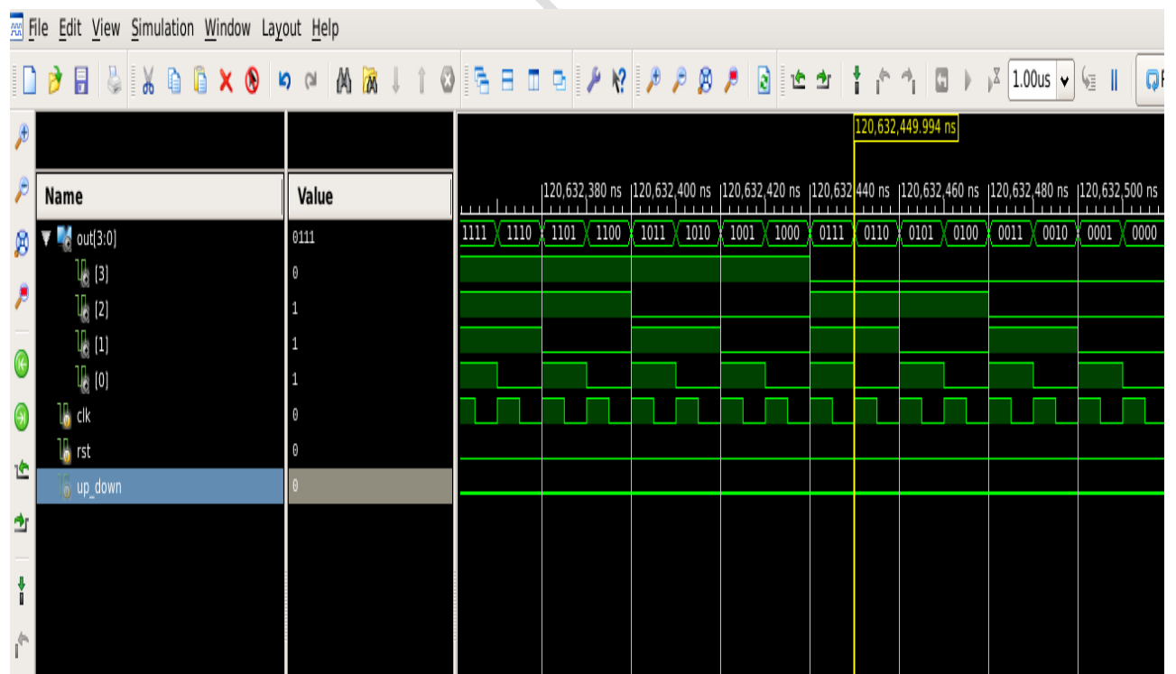
Output waveform:-4 bit up down counter
