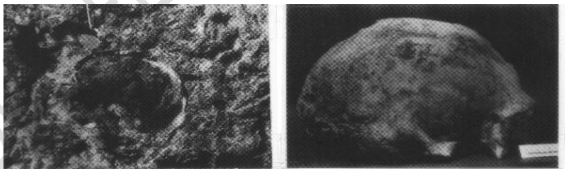
Plate No HE-4 Figure 1.a, Narmada Homo erectus skull in situ in conglomerate bed. b, Narmada Homo erectus skull, after recovery from in situ position
