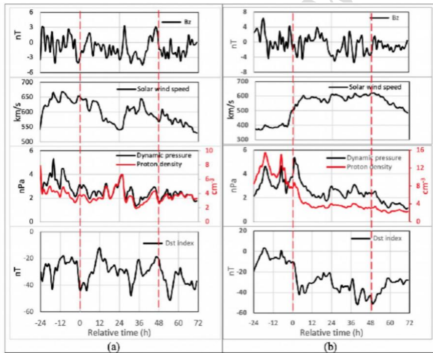
Figure 3: Temporal evolution of the IMF Bz component, solar wind speed, dynamic pressure, proton density, and the Dst index during two recurrent geomagnetic events observed near the minimum phase of Solar Cycle 23. Panel (a) corresponds to the event of 21-22 September 1996 (Bartels rotation 2227), while panel (b) corresponds to the event of 18-19 October 1996 (Bartels rotation 2228). The dashed red lines indicate the beginning and end of each recurrent geomagnetic event.
